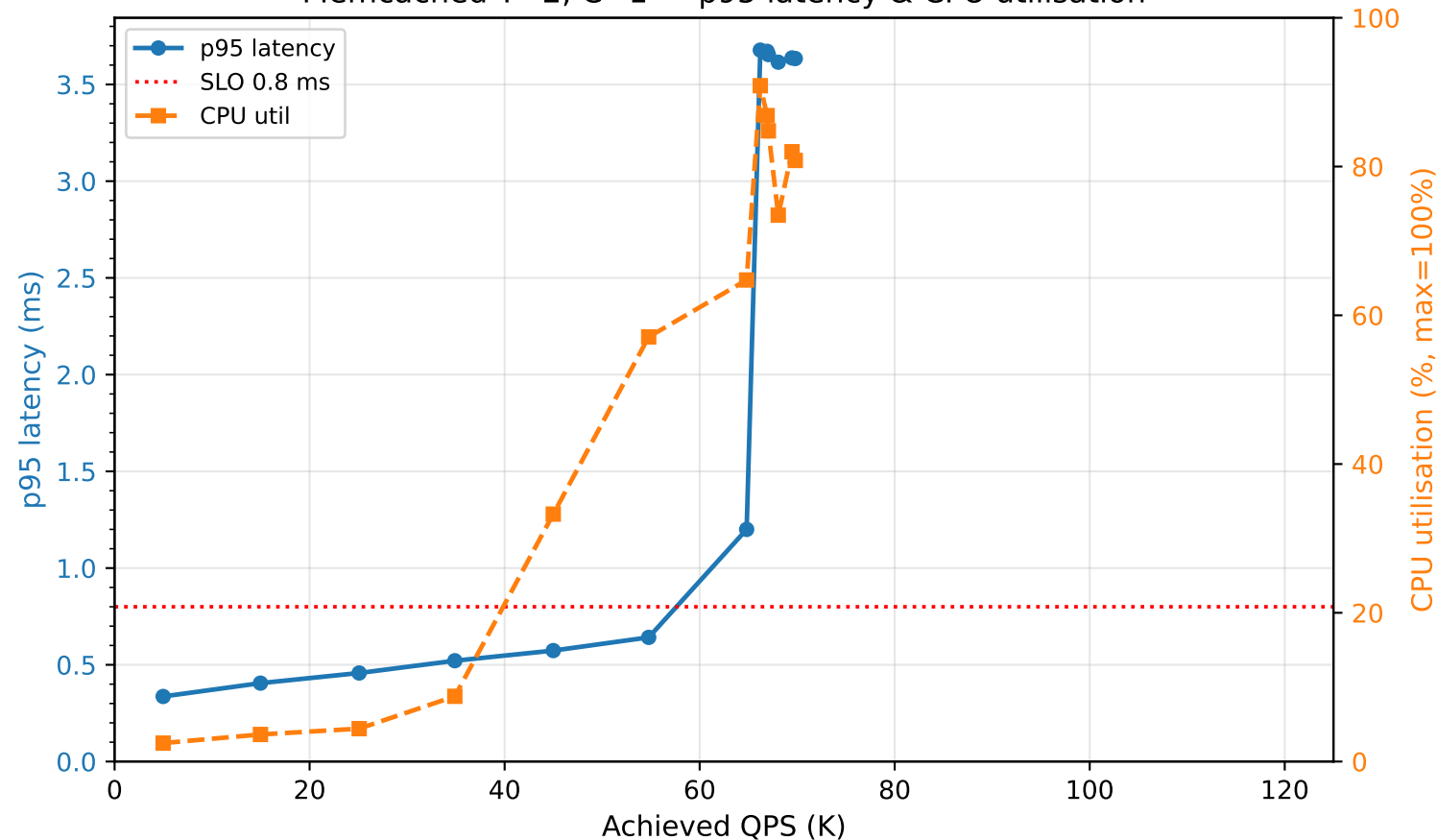
Memcached T=2, C=1 — p95 latency & CPU utilisation
