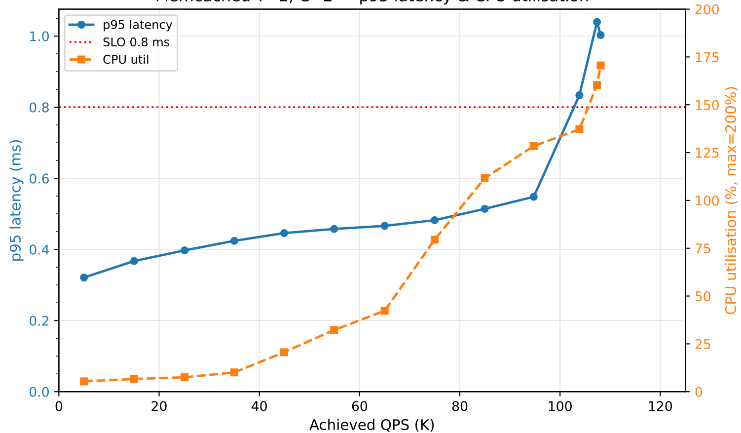
Memcached T=2, C=2 — p95 latency & CPU utilisation
