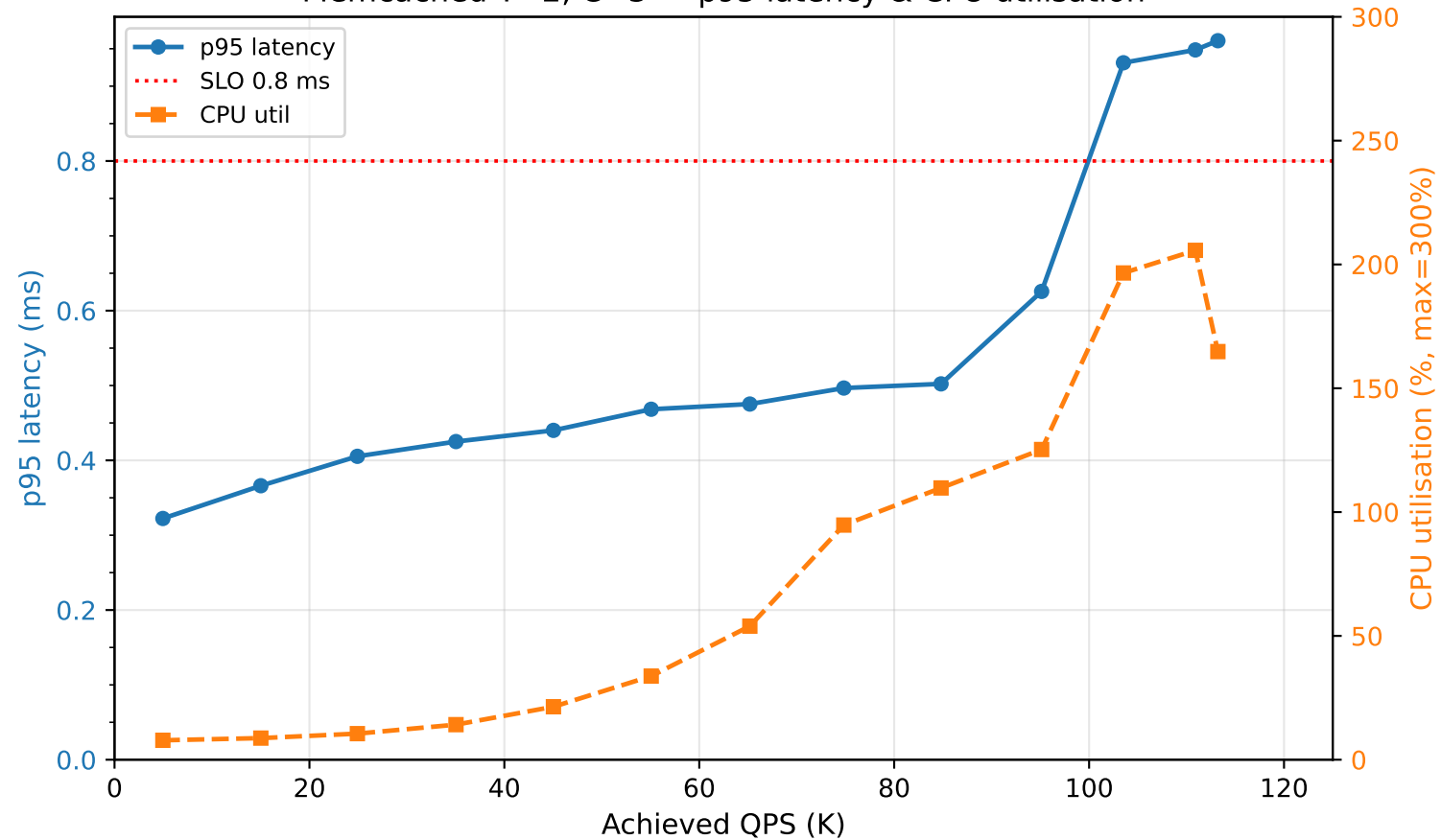
Memcached T=2, C=3 — p95 latency & CPU utilisation
