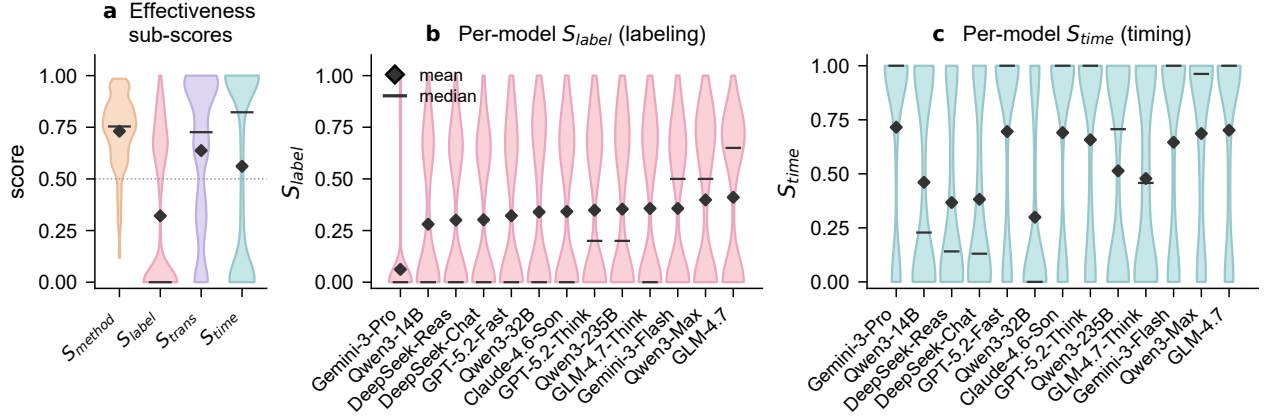
Fig. 3. Failure localization ( \diamond = mean, bar = median). (A) Effectiveness sub-score distributions over all 3,287 protocols, normalized to [0, 1] ( S_{method} = (F_{method} + 1)/2 , 0.5 neutral): S_{label} has the lowest mean (0.32) while S_{method} is high (0.73). (B) Per-model S_{label} distributions (sorted worst-first): the labeling-failure mass concentrates at 0 for every model—most severely for Gemini-3-Pro (mean 0.06)—and 86% of the S_{label}=0 cases are marker–target mismatches, localizing the bottleneck to matching fluorescent markers to the required targets. (C) Per-model S_{time} distributions.
