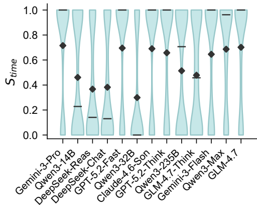
c Per-model S_{time} (timing)
