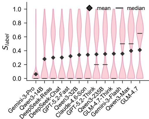
a Effectiveness sub-scores b Per-model S_{label} (labeling)
