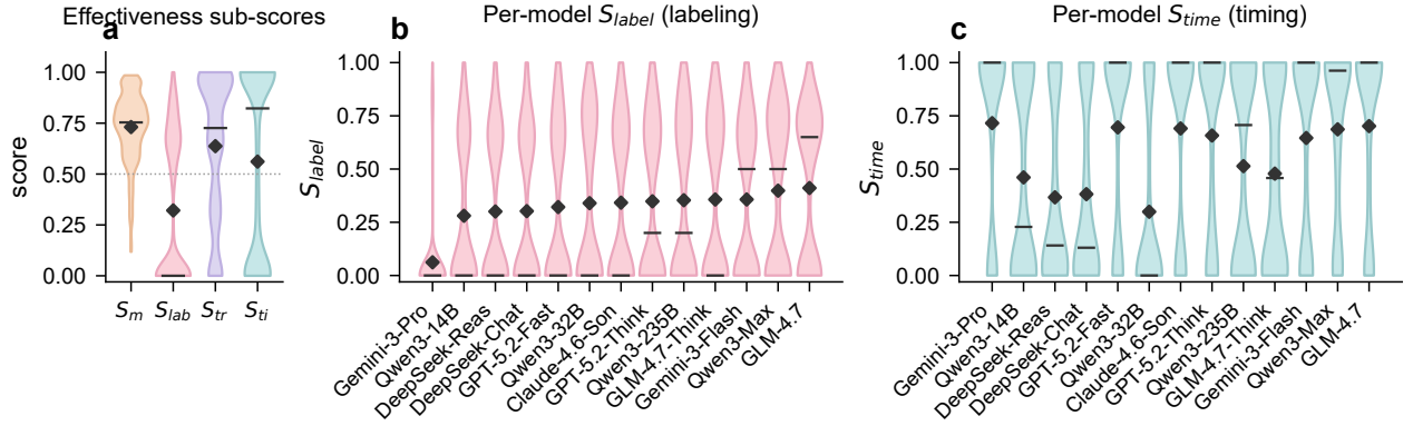
Fig. 3. Failure localization ( \diamond = mean, bar = median). (A) Effectiveness sub-score distributions over all 3,287 protocols, normalized to [0, 1] ( S_{method} = (F_{method} + 1)/2 , 0.5 neutral): S_{label} has the lowest mean (0.32) while S_{method} is high (0.73). (B) Per-model S_{label} distributions (sorted worst-first): the labeling-failure mass concentrates at 0 for every model—most severely for Gemini-3-Pro (mean 0.06)—and 86% of the S_{label}=0 cases are marker–target mismatches, localizing the bottleneck to matching fluorescent markers to the required targets. (C) Per-model S_{time} distributions.
