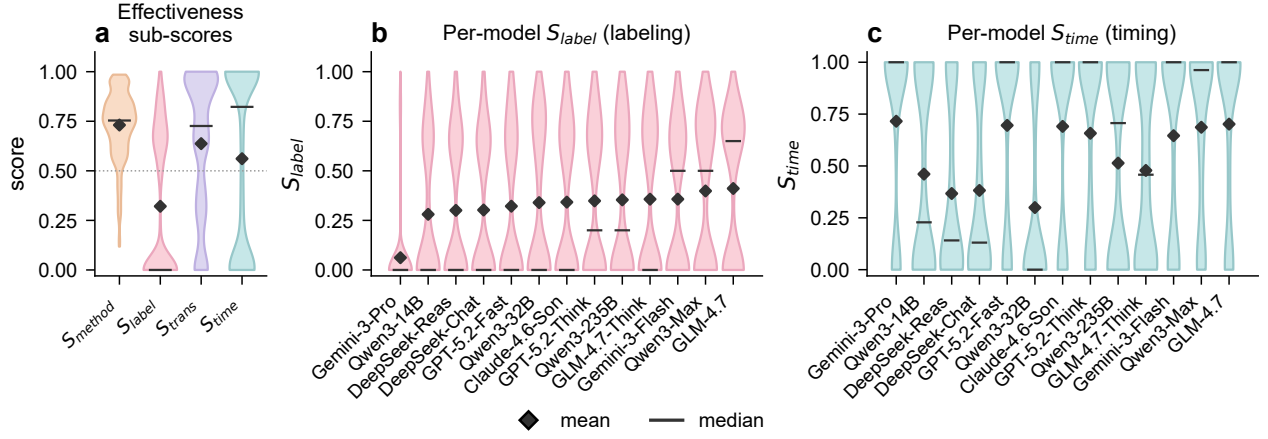
Fig. 3. Failure localization ( \diamond = mean, bar = median). (A) Effectiveness sub-score distributions over all 3,287 protocols, normalized to [0, 1] ( S_{method} = (F_{method} + 1)/2 , 0.5 neutral): S_{label} has the lowest mean (0.32) while S_{method} is high (0.73). (B) Per-model S_{label} distributions (sorted worst-first): the labeling-failure mass concentrates at 0 for every model—most severely for Gemini-3-Pro (mean 0.06)—and 86% of the S_{label}=0 cases are marker–target mismatches, localizing the bottleneck to matching fluorescent markers to the required targets. (C) Per-model S_{time} distributions.
