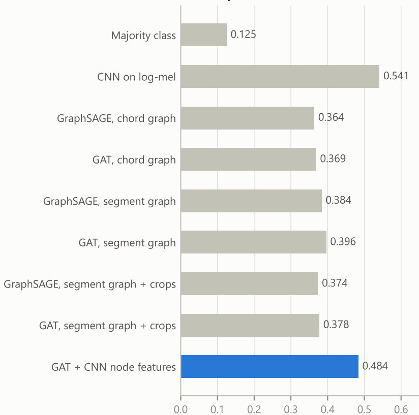
Accuracy
