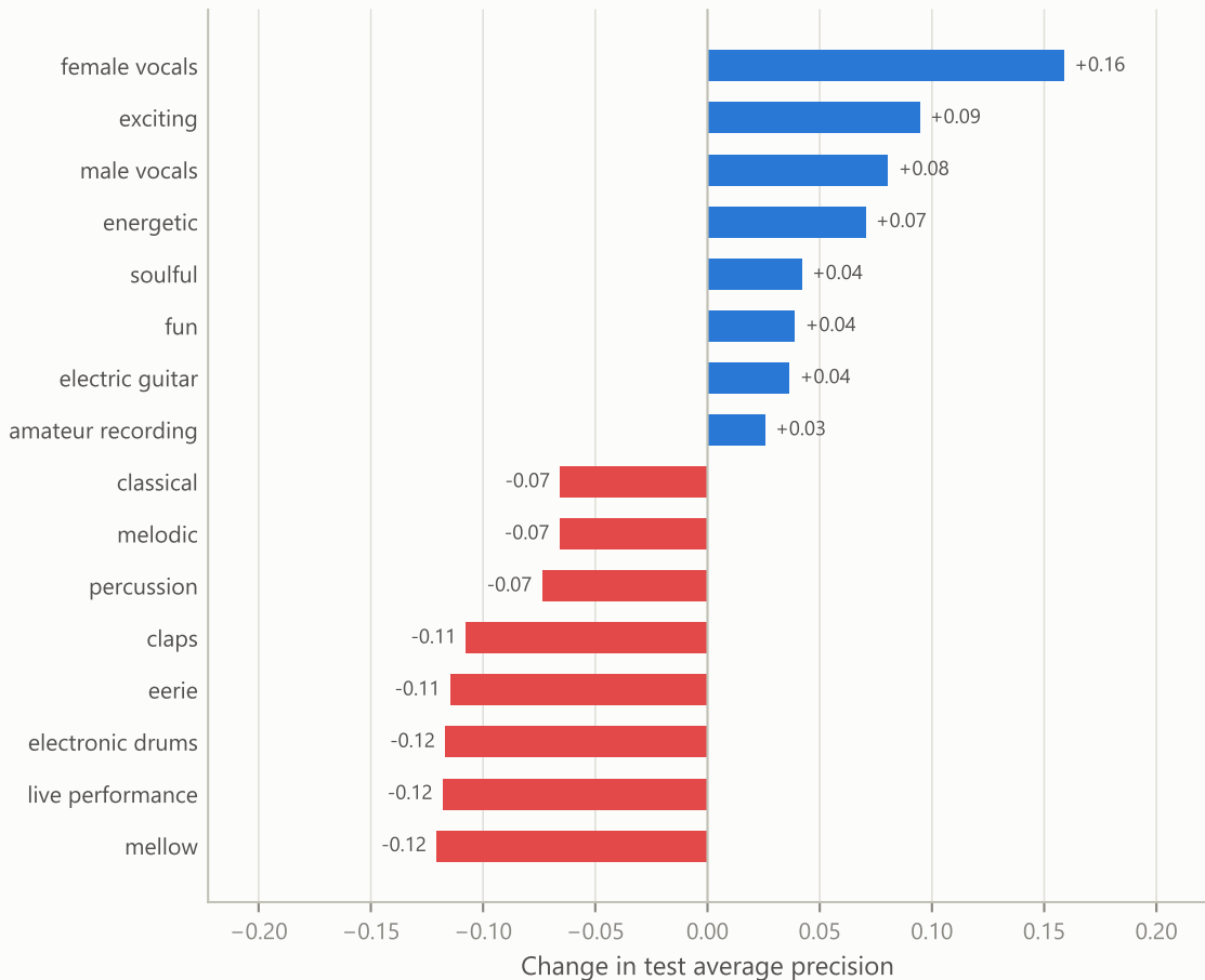
Adding the audio graph: early concat minus BERT only
