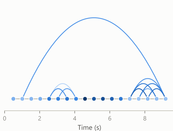
Segment graph, nodes shaded by attention
