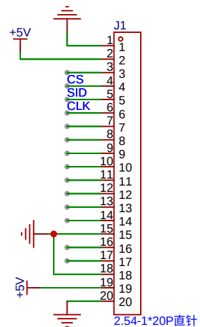
Lcd12864排针
