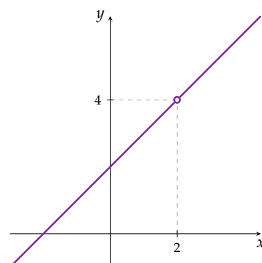
Figure 1 The graph of f(x) , where the function is undefined at x = 2 .
