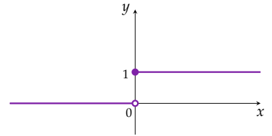
Figure 3 The Heaviside function H(x) , where it breaks at x = 0 .
