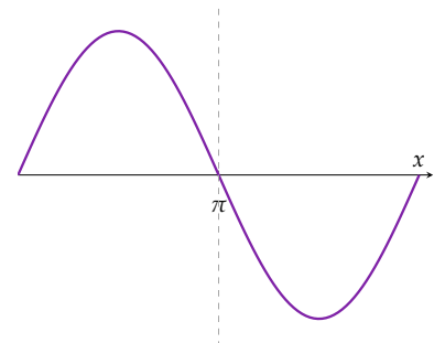
Figure 2 \sin(x) at [0, 2\pi]
