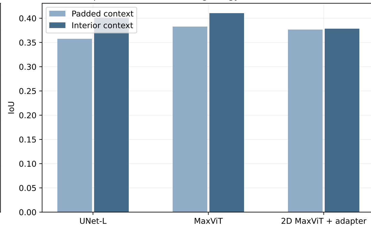
Spatial strata (different geology; not a causal test)
