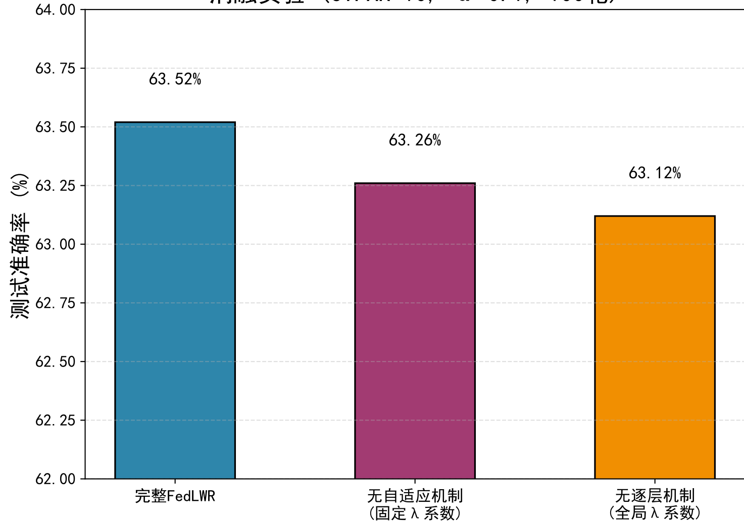
消融实验 (CIFAR-10, \alpha=0.1 , 100轮)
