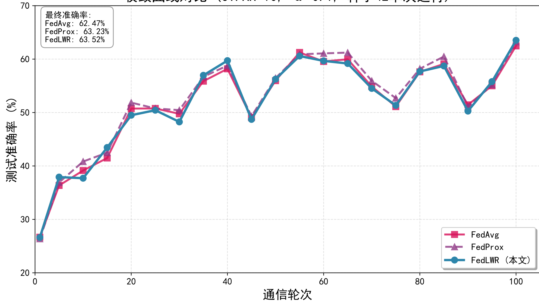
收敛曲线对比 (CIFAR-10, \alpha=0.1 , 种子42单次运行)
