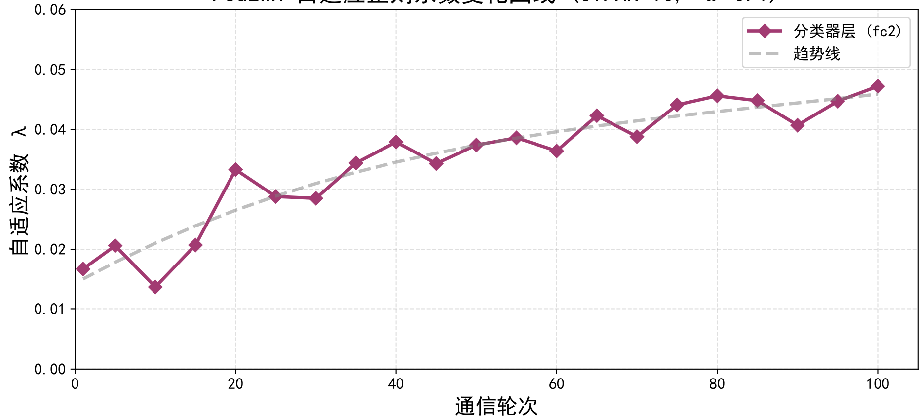
FedLWR 自适应正则系数变化曲线 (CIFAR-10, \alpha=0.1 )
