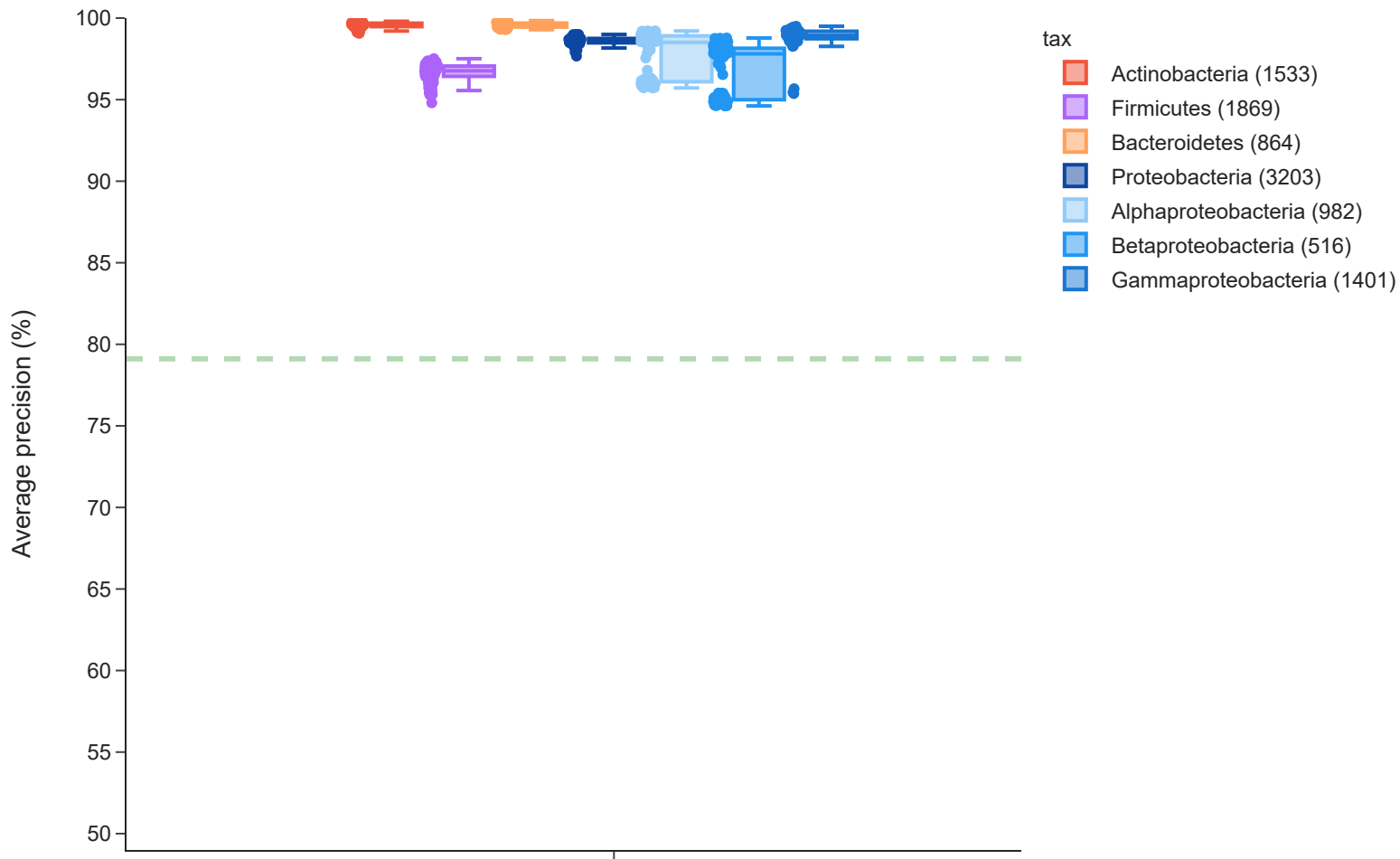
Average precision RF
