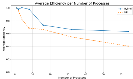
Figure: Average M-Step Efficiency Comparison between Pure MPI and Hybrid approach.
