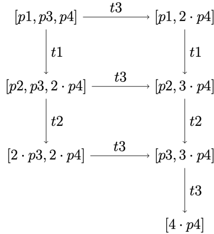
Figure 33: Reachability Graph of the Example Petri Net
