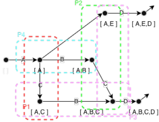
Figure 42: Identified Regions from the Transition System
