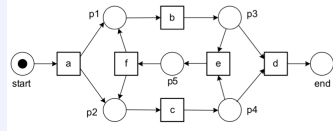
Figure 46: Petri net for Exercise 4
