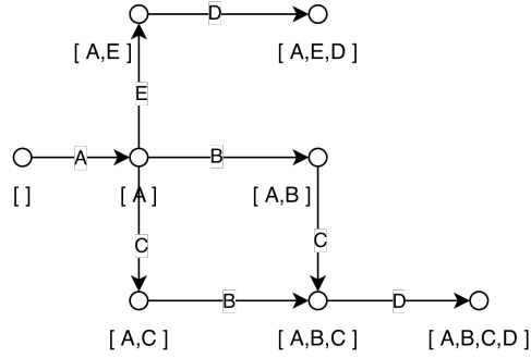
Figure 41: Transition System using Past with Set Abstraction
