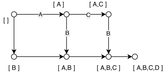
Figure 38: Transition System using Past with Multiset Abstraction
