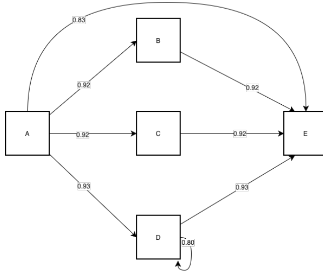
Figure 36: Dependency Graph for the Event Log L
