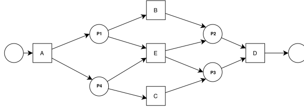
Figure 43: Petri Net Discovered using the Region Based Miner
