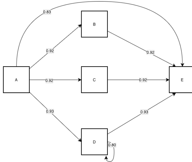
Figure 50: Dependency Graph for the Event Log L
