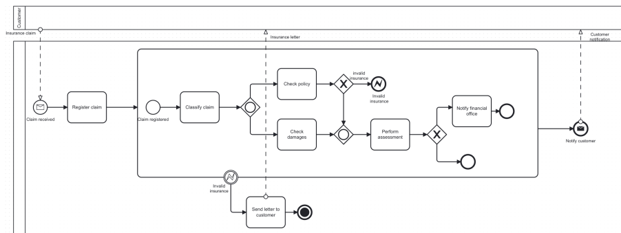
Figure 40: Solution for Exercise 10
