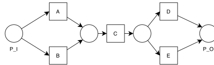
Figure 48: Petri Net Discovered using the Alpha Miner
