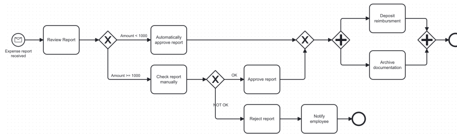
Figure 38: Solution for Exercise 8
