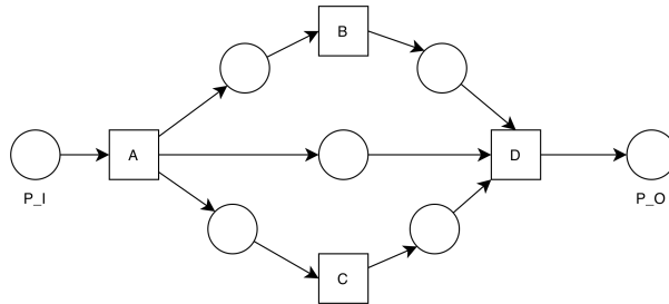
Figure 49: Petri Net Discovered using the Alpha Miner
