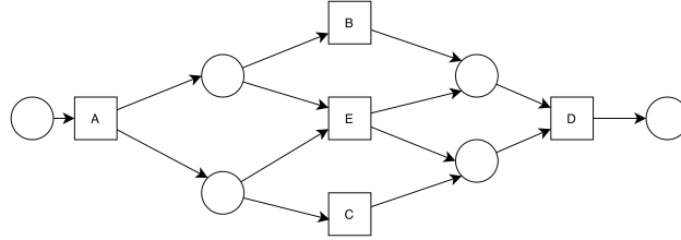
Figure 46: Petri Net Discovered using the Alpha Miner
