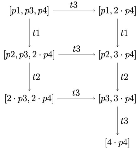
Figure 45: Reachability Graph of the Example Petri Net
