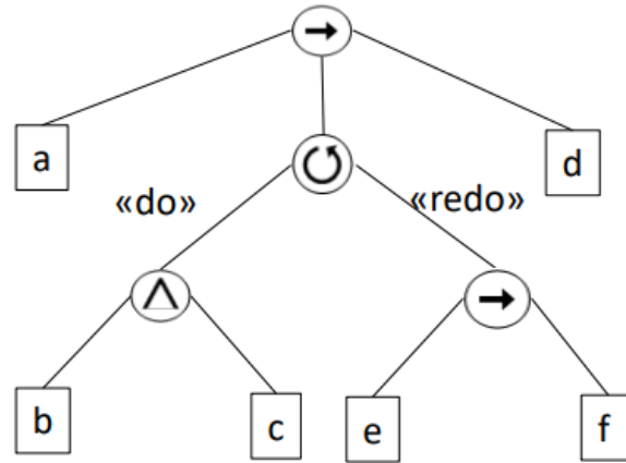
Figure 29: Example of Process Tree
