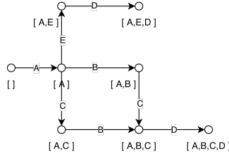
Figure 56: Transition System using Past with Set Abstraction
