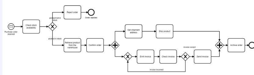
Figure 42: Example Process for Quantitative Analysis Exercises
