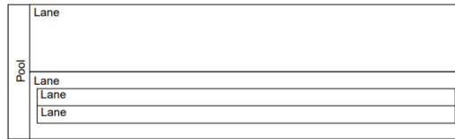
Figure 8: Pools and Lanes in BPMN
