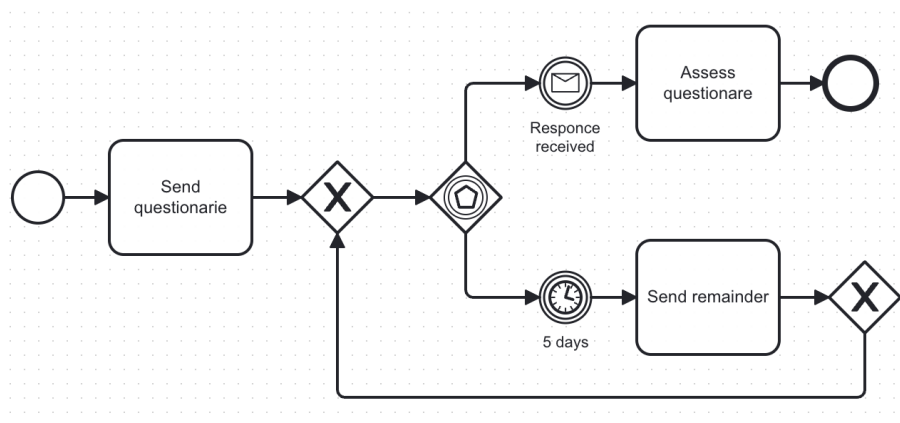
Figure 36: Solution for Exercise 6
