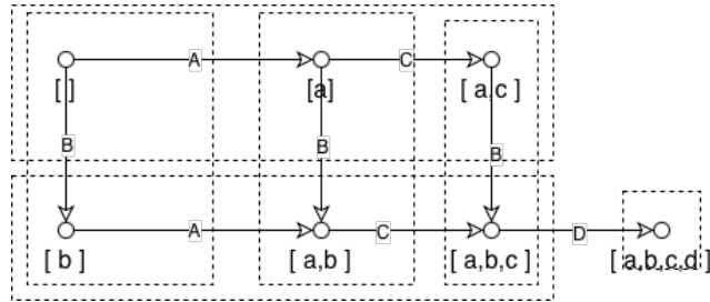
Figure 54: Identified Regions from the Transition System
