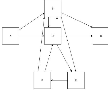
Figure 61: Directly-Follows Graph for the Event Log L
