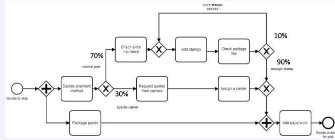
Figure 43: Example Process for Quantitative Analysis Exercise 2
