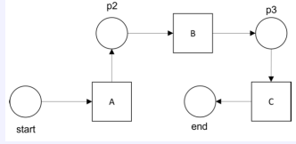
Figure 69: Petri net for Exercise 5
