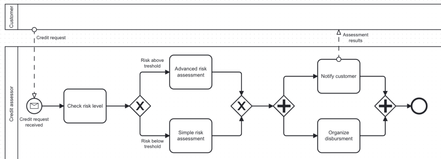
Figure 39: Solution for Exercise 9
