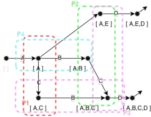
Figure 57: Identified Regions from the Transition System
