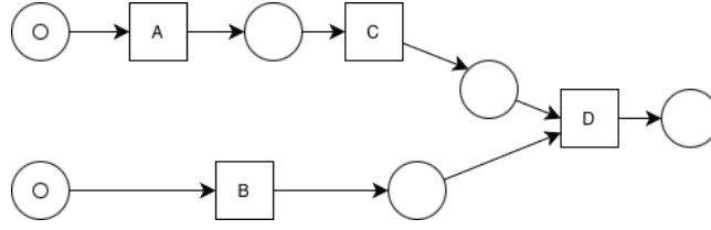
Figure 55: Petri Net Derived from the Transition System
