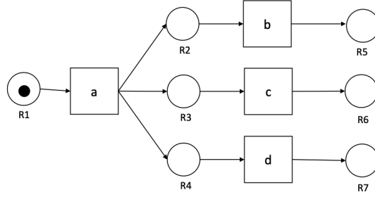
Figure 60: Petri Net Discovered using the Region Based Miner
