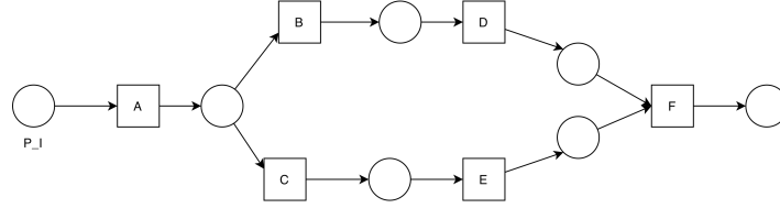
Figure 66: Petri net for Exercise 2
