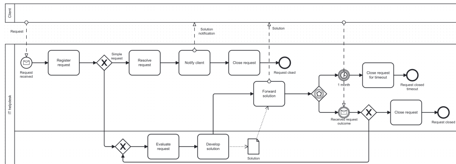
Figure 37: Solution for Exercise 7
