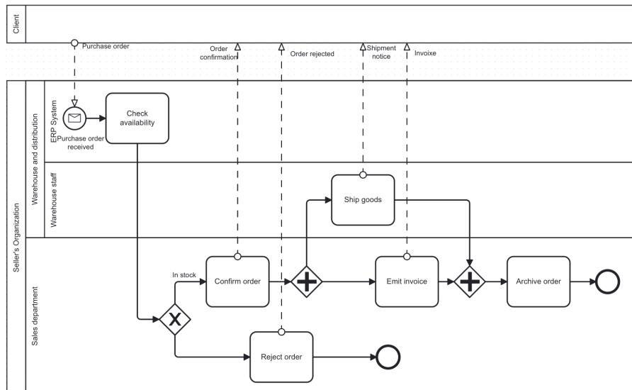
Figure 35: Solution for Exercise 5
