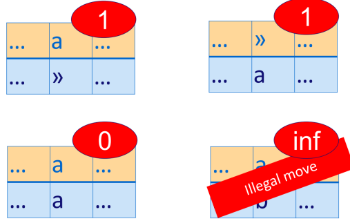
Figure 30: Example of an alignments
