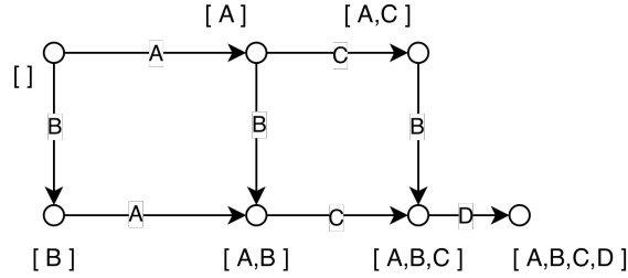
Figure 53: Transition System using Past with Multiset Abstraction
