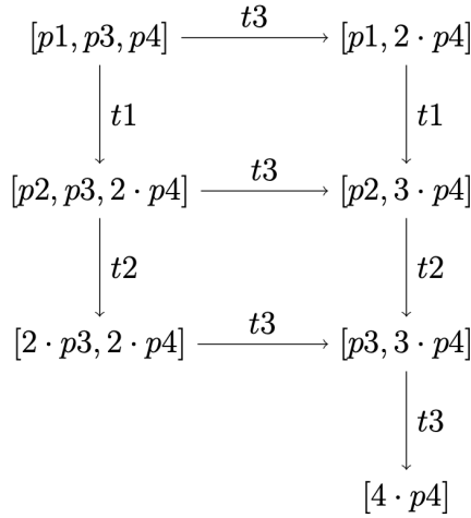
Figure 34: Reachability Graph of the Example Petri Net
