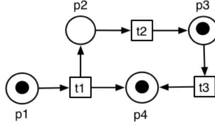
Figure 33: Example Petri Net for Property Analysis
