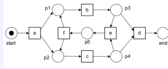
Figure 52: Petri net for Exercise 4
