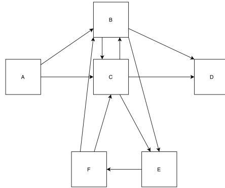
Figure 45: Directly-Follows Graph for the Event Log L
