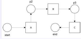
Figure 53: Petri net for Exercise 5
