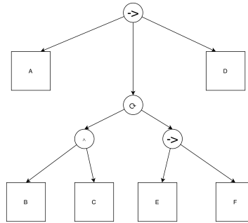
Figure 48: Process Model Discovered using the Inductive Miner
