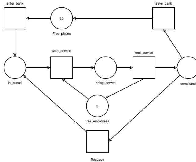
Figure 33: Petri Net Model of the Bank Process
