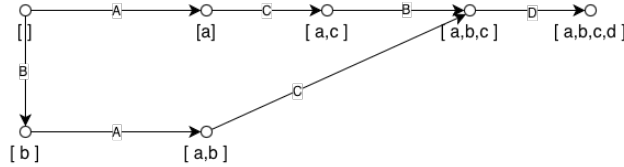
Figure 37: Transition System using Past with Multiset Abstraction
