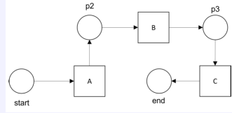
Figure 43: Petri net for Exercise 5
