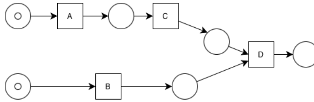
Figure 39: Petri Net Derived from the Transition System
