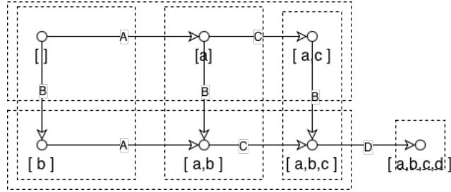
Figure 38: Identified Regions from the Transition System
