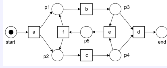
Figure 50: Petri net for Exercise 4
