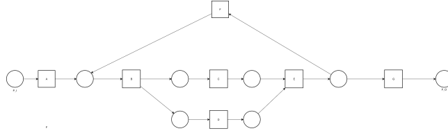
Figure 35: Petri Net Discovered using the Alpha Miner
