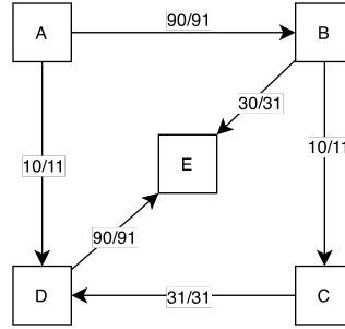
Figure 48: Dependency Graph for the Event Log L_2
