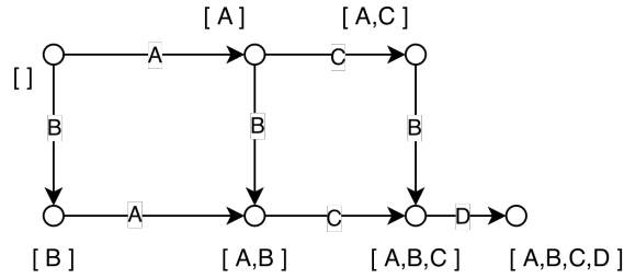
Figure 50: Transition System using Past with Multiset Abstraction
