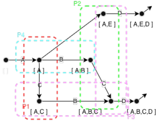
Figure 54: Identified Regions from the Transition System
