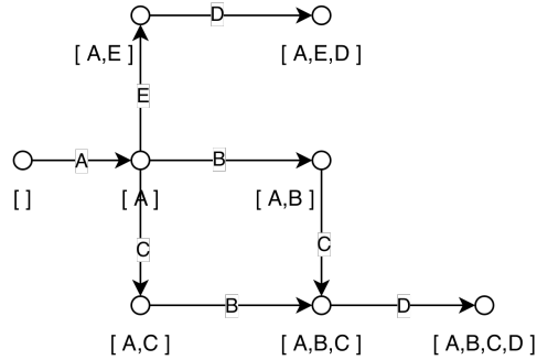
Figure 53: Transition System using Past with Set Abstraction
