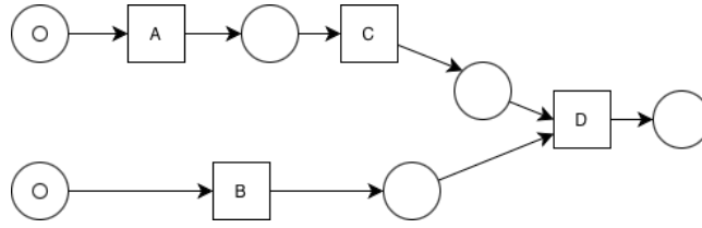
Figure 52: Petri Net Derived from the Transition System
