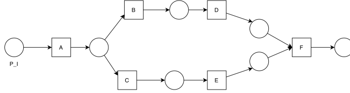
Figure 61: Petri net for Exercise 2
