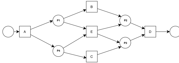
Figure 55: Petri Net Discovered using the Region Based Miner
