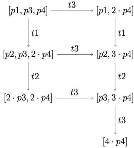
Figure 43: Reachability Graph of the Example Petri Net
