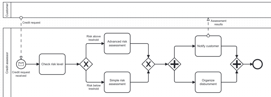
Figure 38: Solution for Exercise 9
