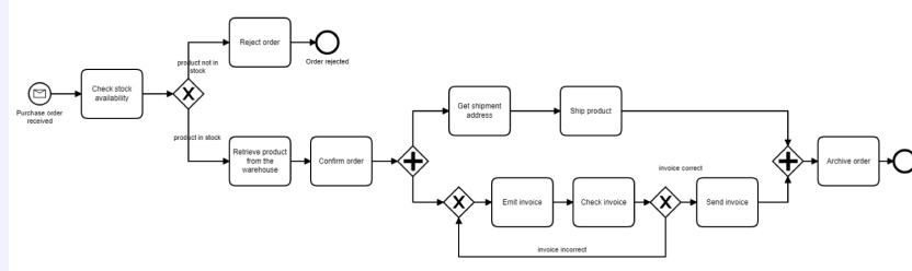
Figure 40: Example Process for Quantitative Analysis Exercises
