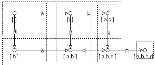
Figure 51: Identified Regions from the Transition System
