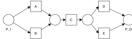
Figure 46: Petri Net Discovered using the Alpha Miner
