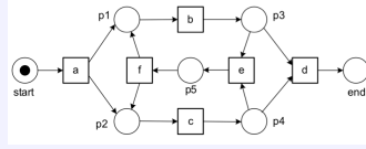
Figure 63: Petri net for Exercise 4
