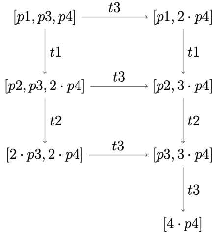
Figure 44: Reachability Graph of the Example Petri Net
