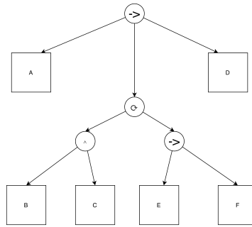
Figure 63: Process Model Discovered using the Inductive Miner
