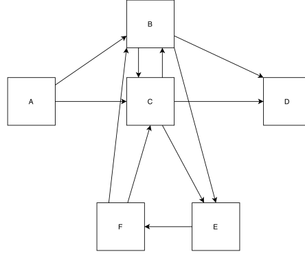
Figure 60: Directly-Follows Graph for the Event Log L
