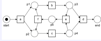
Figure 67: Petri net for Exercise 4
