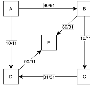
Figure 50: Dependency Graph for the Event Log L_2
