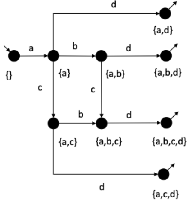
Figure 58: Transition System using Past with Set Abstraction
