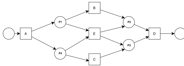
Figure 57: Petri Net Discovered using the Region Based Miner
