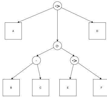
Figure 64: Process Model Discovered using the Inductive Miner
