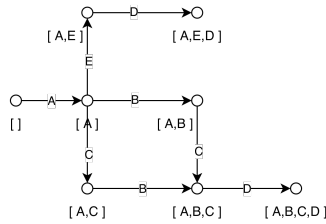
Figure 56: Transition System using Past with Set Abstraction
