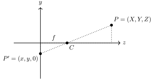
Figure 12: Perspective Projection
