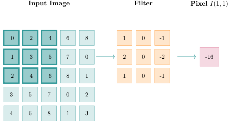
Figure 6: Example of convolution between an image and a filter.
