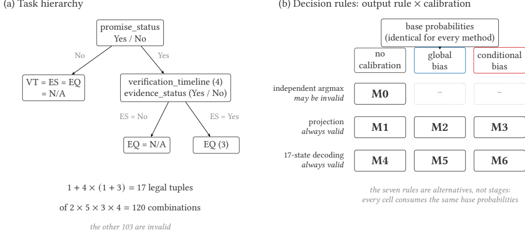
Figure 1: The task hierarchy and the seven decision rules. Panel (b) is the 2 \times 3 design of Section 6: either structured output rule may be combined with any of the three calibration settings, and the cells are alternatives rather than stages. All of them consume identical base probabilities; projection and 17-state decoding guarantee a legal tuple, whereas independent argmax does not, which is why its row has only the uncalibrated cell.
