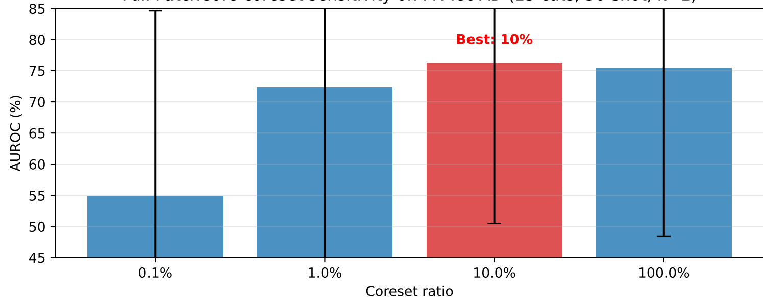
Full PatchCore coreset sensitivity on MVTec AD (15 cats, 50-shot, k=1)
