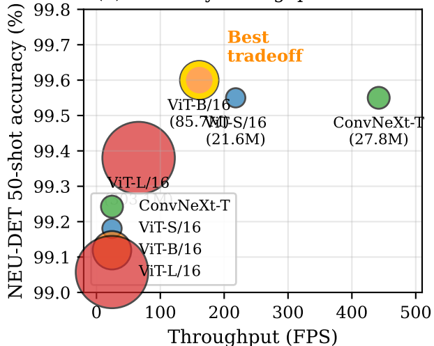
(b) Accuracy-throughput tradeoff
