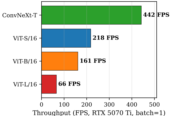
(a) Inference throughput by backbone
