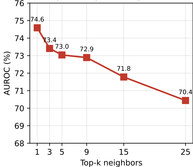
Top-k sweep (memory=5000)
