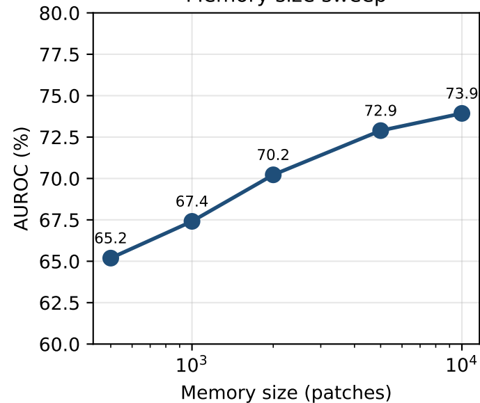
Memory size sweep
