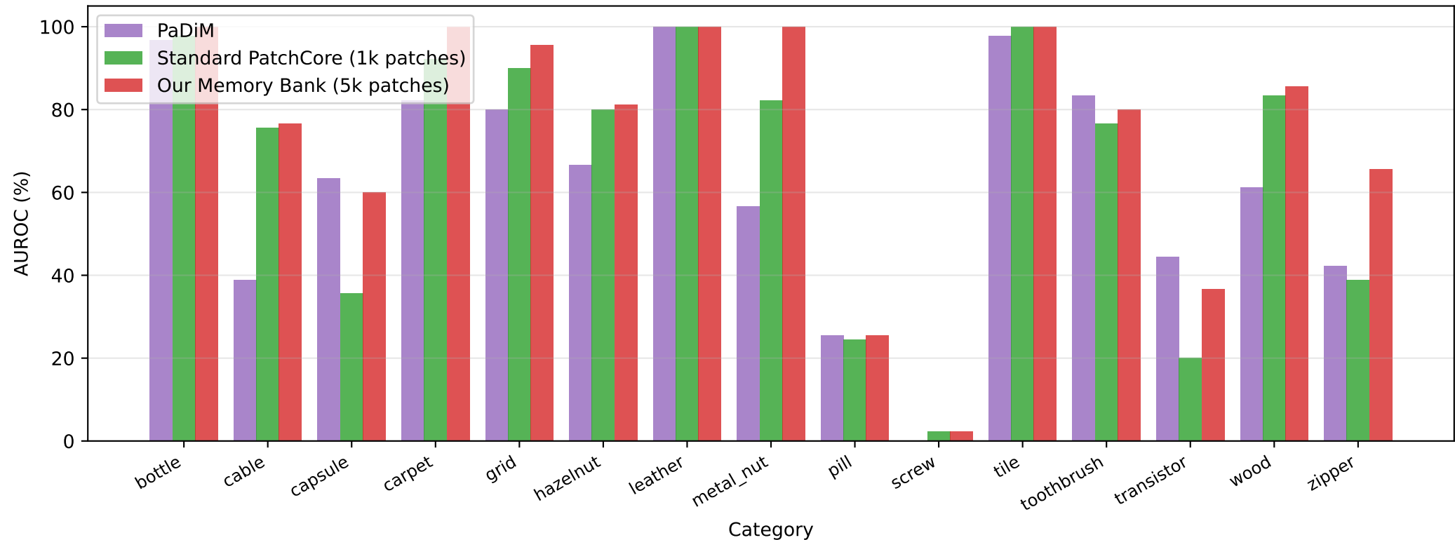
MVTec AD full 15 categories: AUROC comparison at 50-shot, 3 seeds
