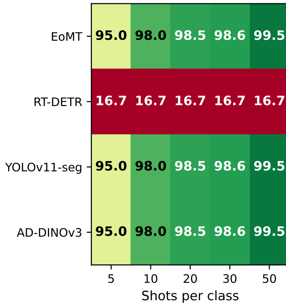
ConvNeXt-T
