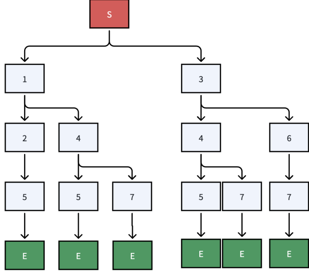
Figure 4: The six valid paths on a 3 \times 3 grid with S = (0, 0) and E = (2, 2) .
