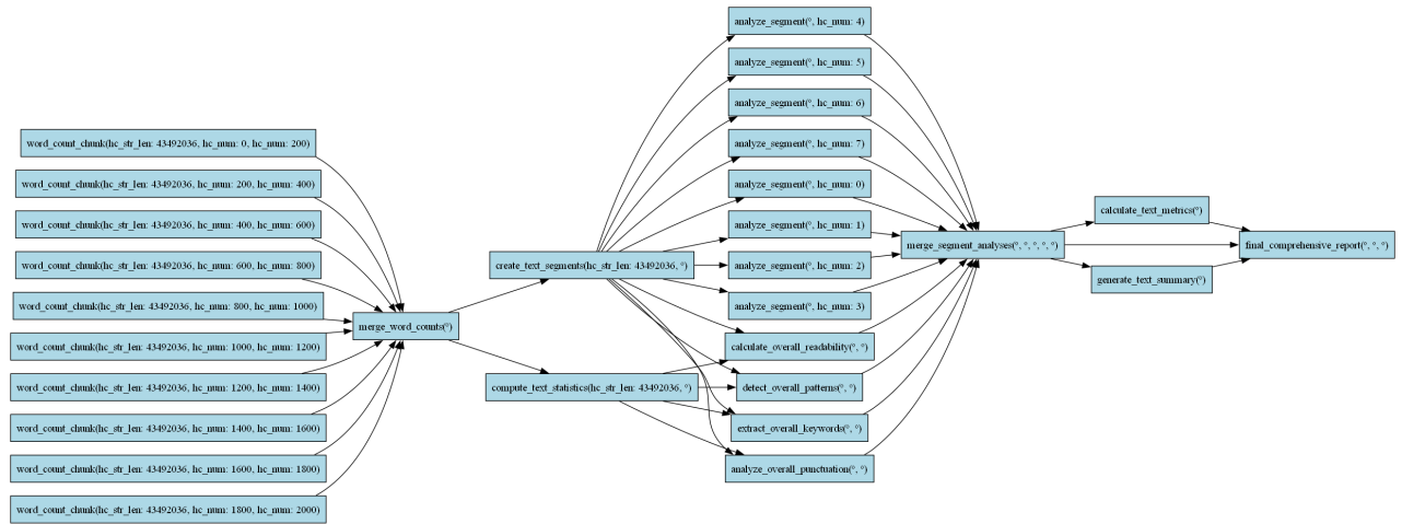
Figure 3.4: DAG Visualization Feature for a Text Analysis Workflow
