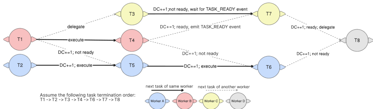
Figure 3.6: Choreographed Scheduling Example
