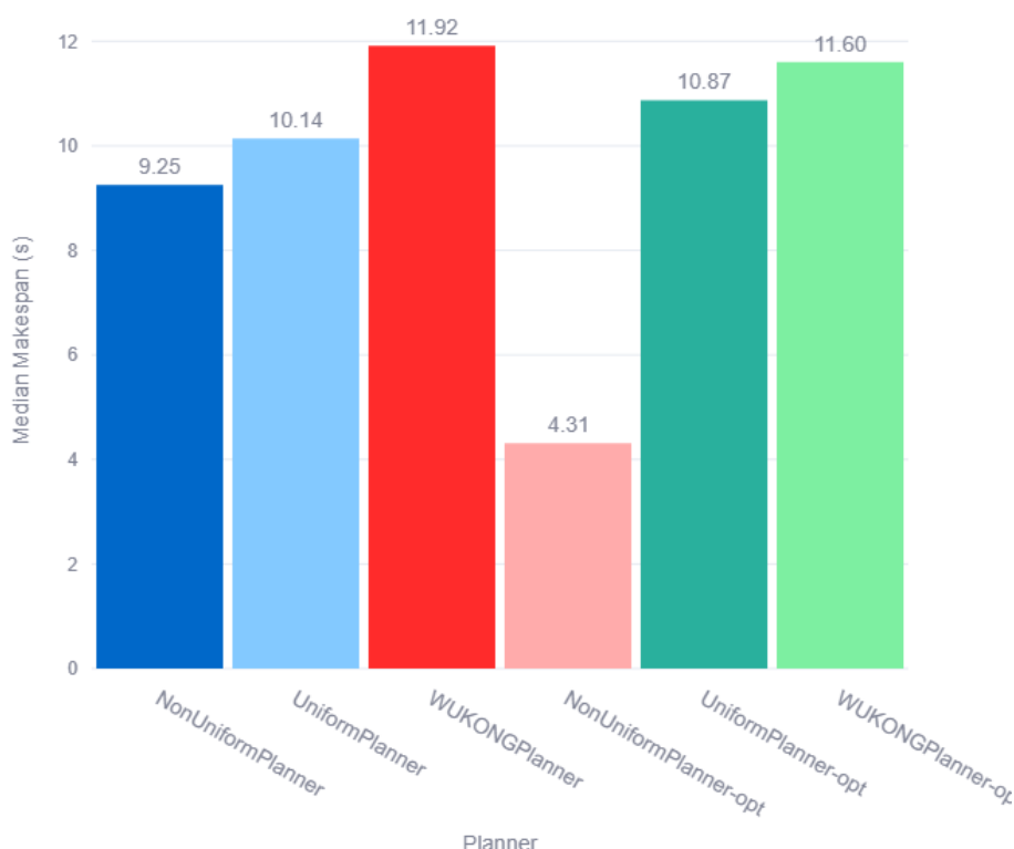
Figure 4.8: Makespan comparison
