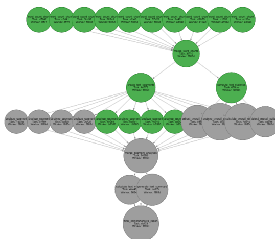
Figure 3.6: Workflow Real-time Dashboard
