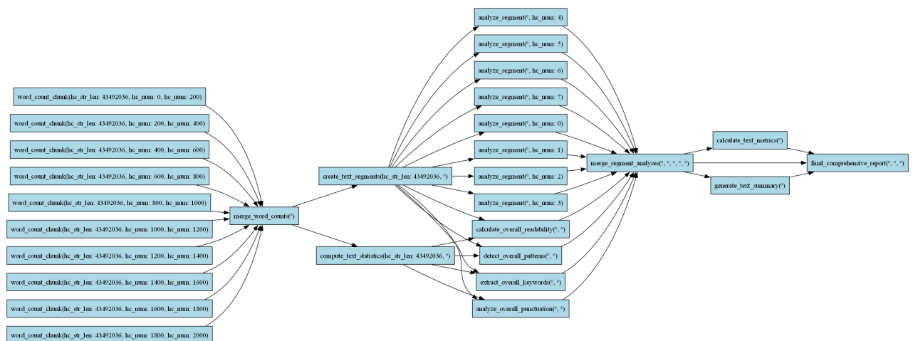
Figure 3.5: DAG Visualization Feature for a Text Analysis Workflow
