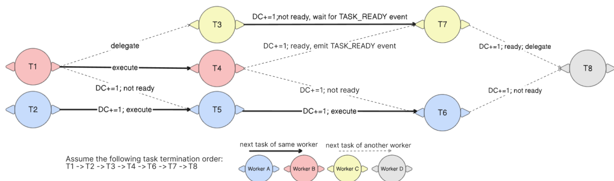
Figure 3.4: Choreographed Scheduling Example
