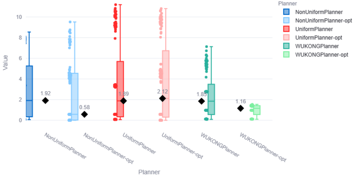
Figure 4.3: Waiting for dependencies distribution between planners
