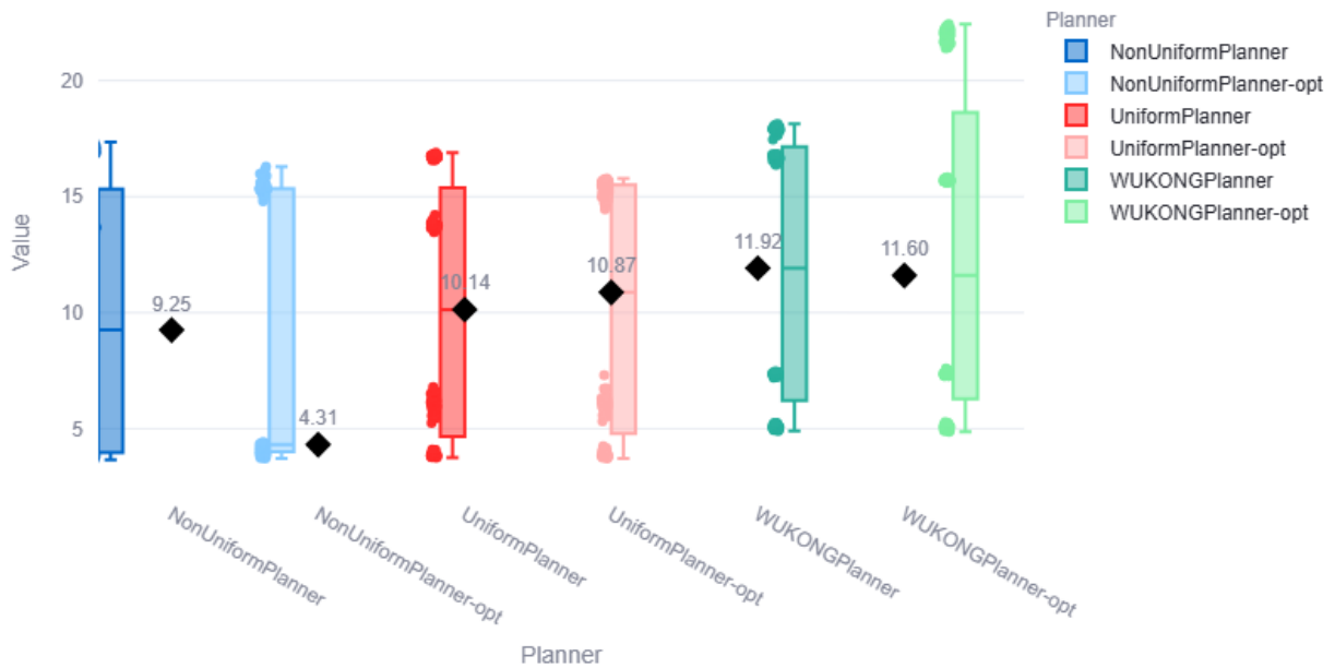
Figure 4.2: Makespan distribution between planners
