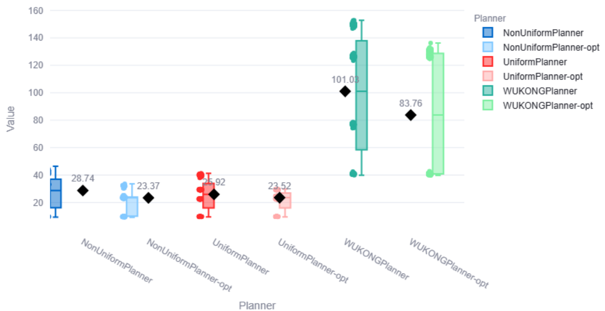
Figure 4.4: Worker startup time distribution between planners
