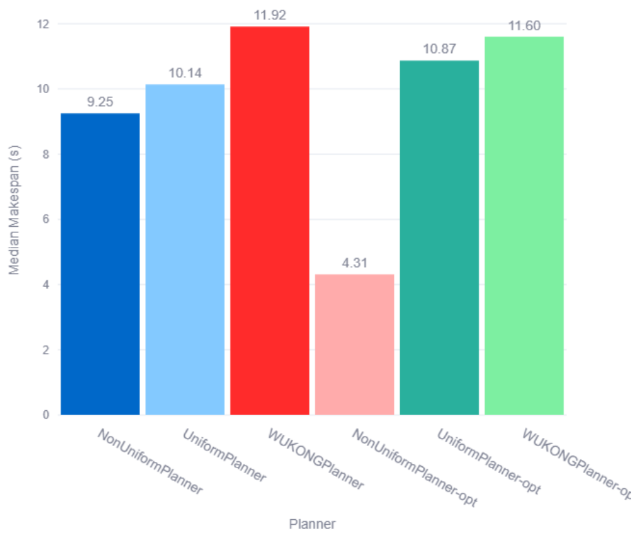
Figure 4.8: Makespan comparison
