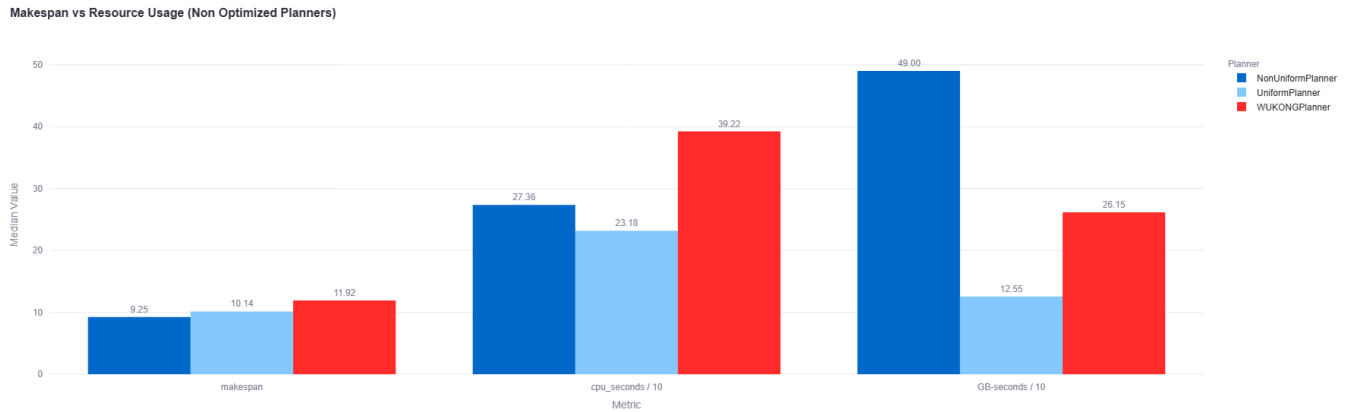
Figure 4.8: Makespan vs Resource Usage comparison to WUKONG
