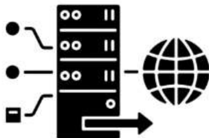
FORWARD PROXIES
