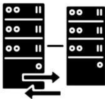
REVERSE PROXIES
