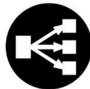
LOAD BALANCERS
