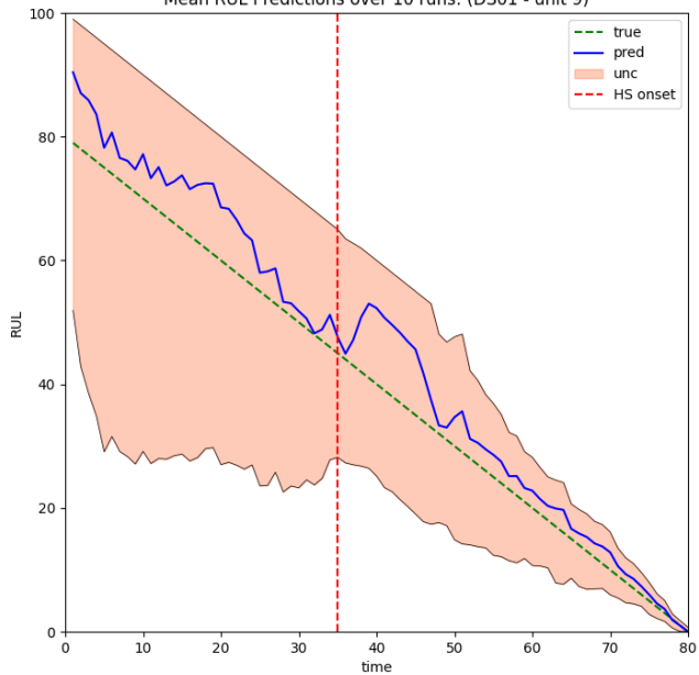
Mean RUL Predictions over 10 runs: (DS01 - unit 9)
