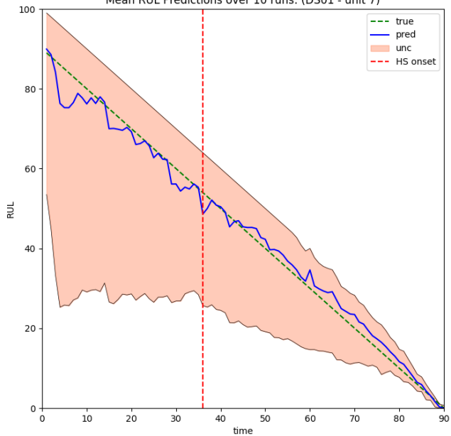
Mean RUL Predictions over 10 runs: (DS01 - unit 7)
