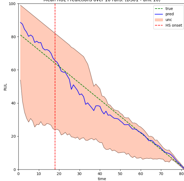
Mean RUL Predictions over 10 runs: (DS01 - unit 10)
