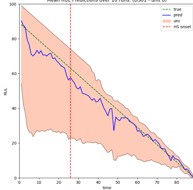
Mean RUL Predictions over 10 runs: (DS01 - unit 8)
