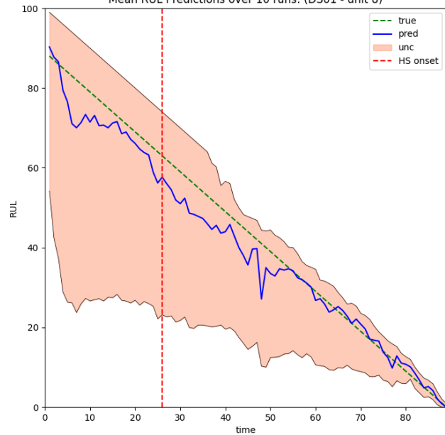
Mean RUL Predictions over 10 runs: (DS01 - unit 8)
