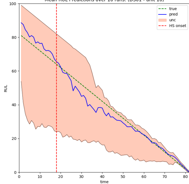
Mean RUL Predictions over 10 runs: (DS01 - unit 10)
