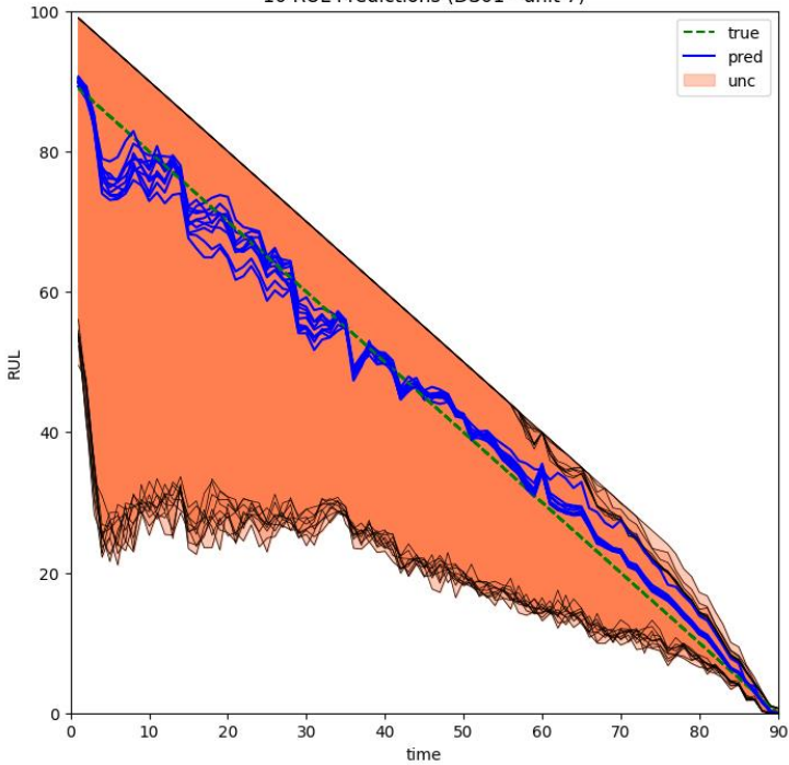
10 RUL Predictions (DS01 - unit 7)
