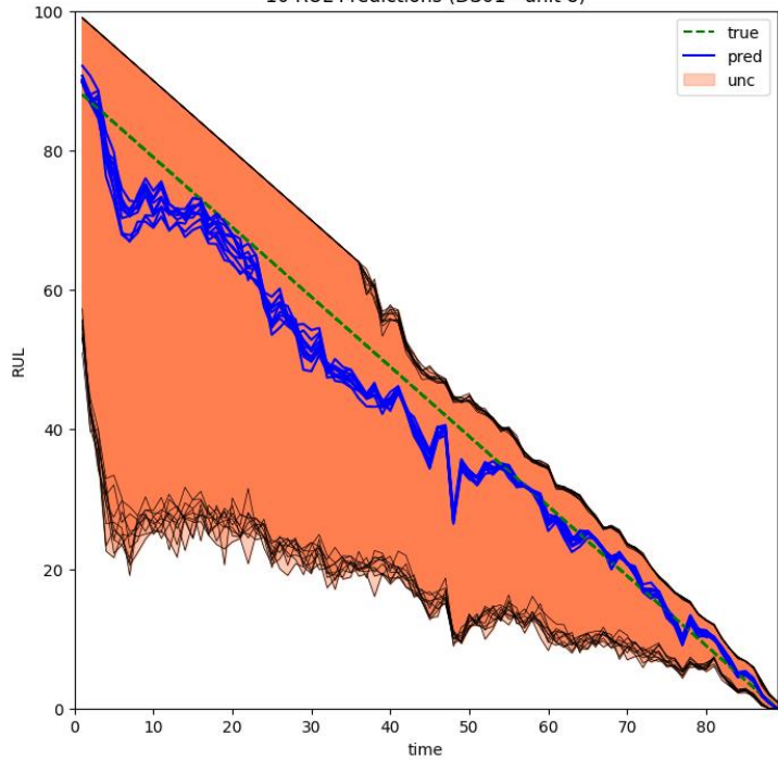
10 RUL Predictions (DS01 - unit 8)
