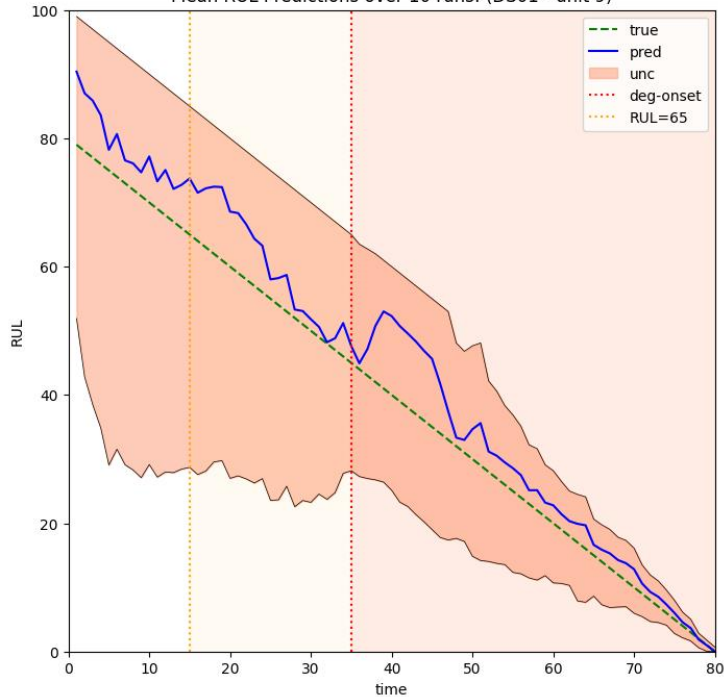
Mean RUL Predictions over 10 runs: (DS01 - unit 9)
