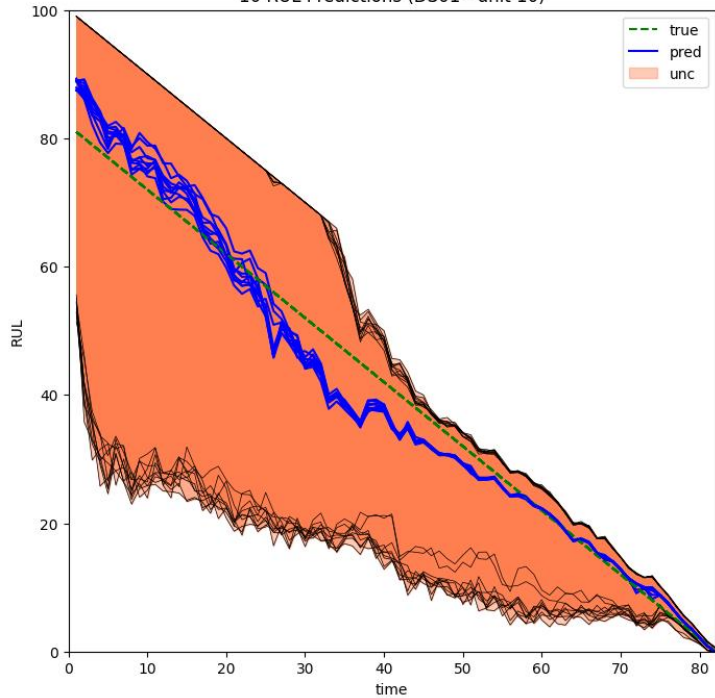
10 RUL Predictions (DS01 - unit 10)
