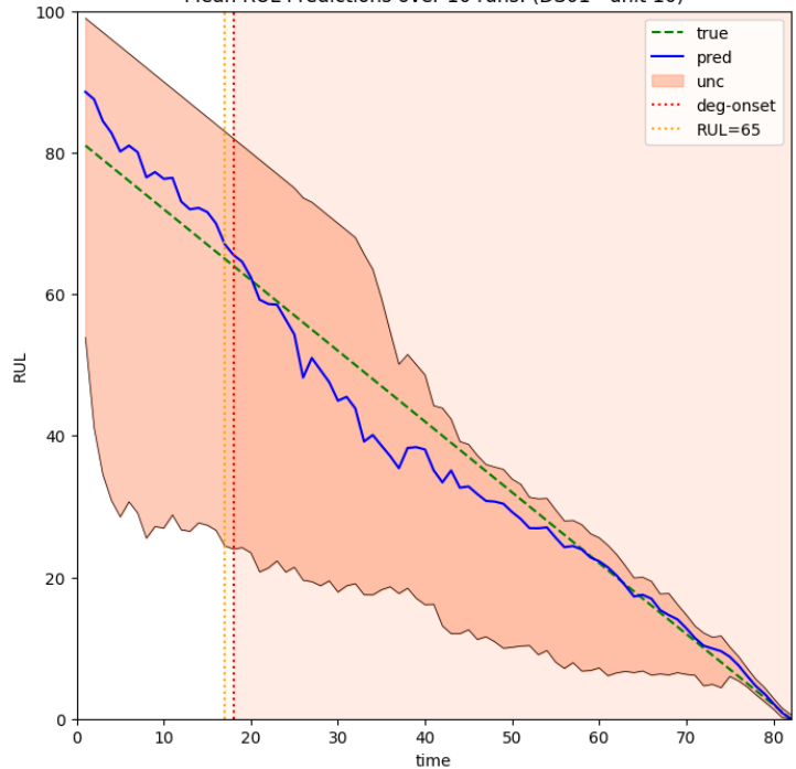
Mean RUL Predictions over 10 runs: (DS01 - unit 10)
