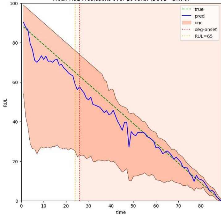
Mean RUL Predictions over 10 runs: (DS01 - unit 8)
