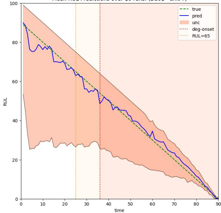
Mean RUL Predictions over 10 runs: (DS01 - unit 7)
