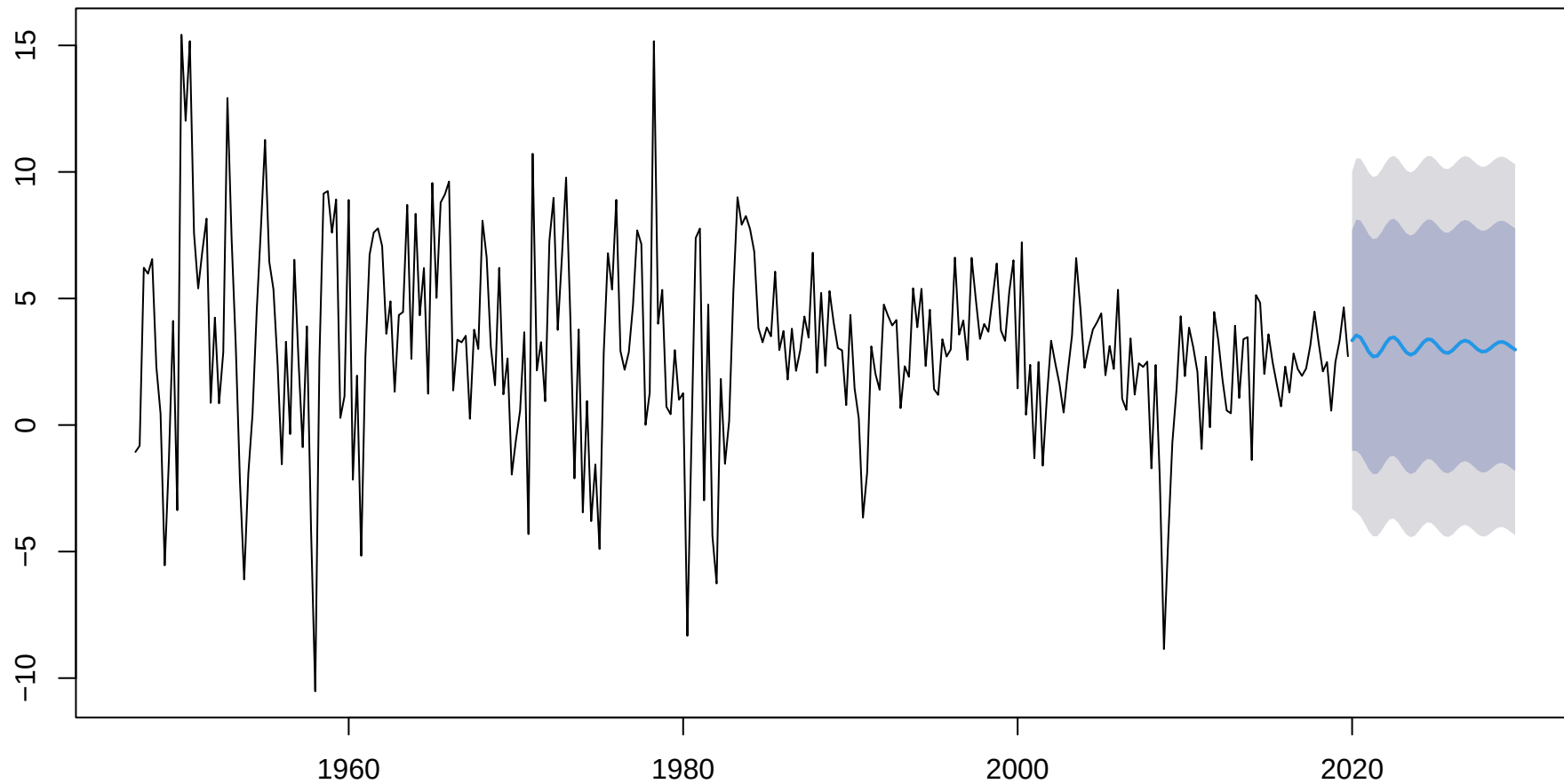
Forecasts from ARIMA(3,0,2) with non-zero mean
