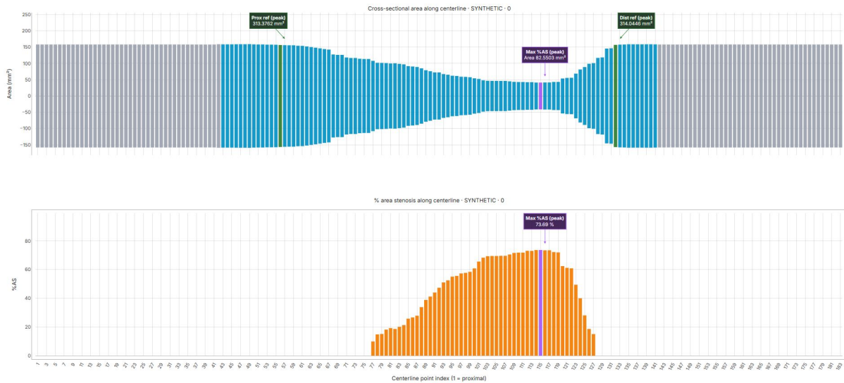
Figure 3.9: Longitudinal area and %AS profiles along the stenosis synthetic tube.
