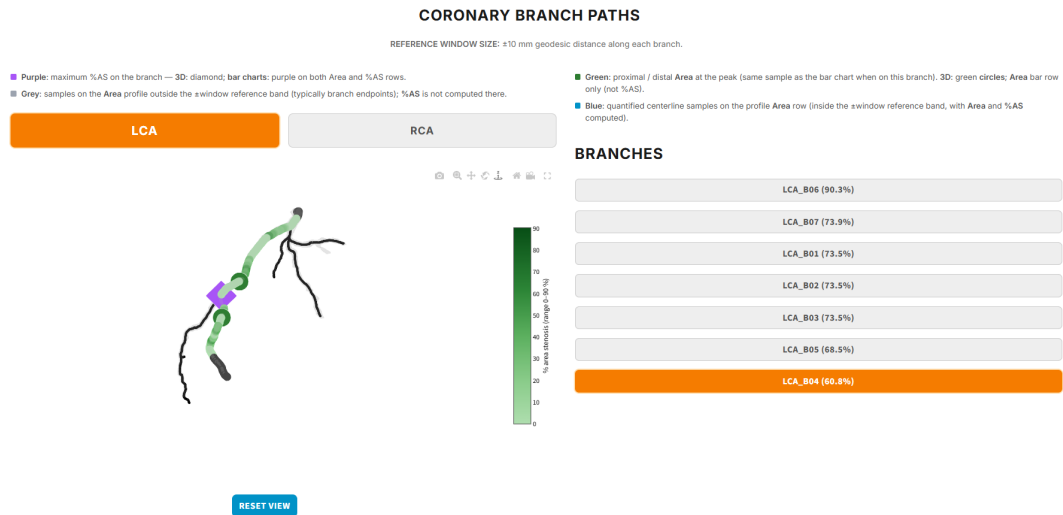
Figure 3.15: Dashboard Module 4: branch-level three-dimensional path highlighting and longitudinal metric profiles.
