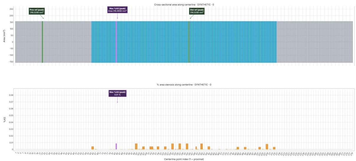
Figure 3.7: Longitudinal area and %AS profiles along the healthy synthetic tube.
