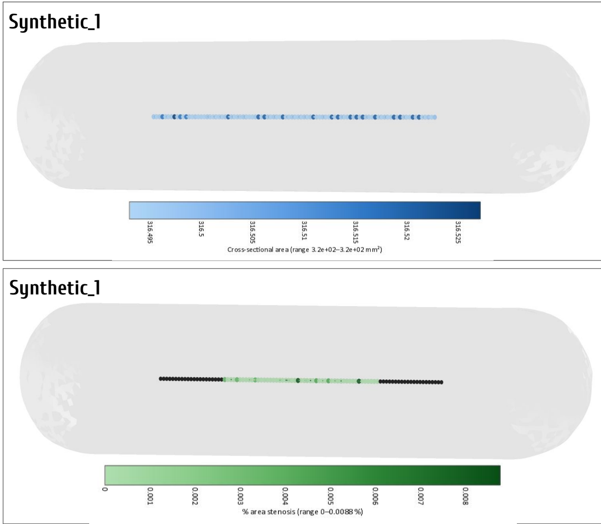
Figure 3.8: Three-dimensional area and %AS colormaps for the healthy synthetic tube.
